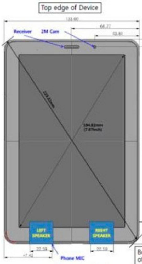
Figure 11-1 Front View of Device
