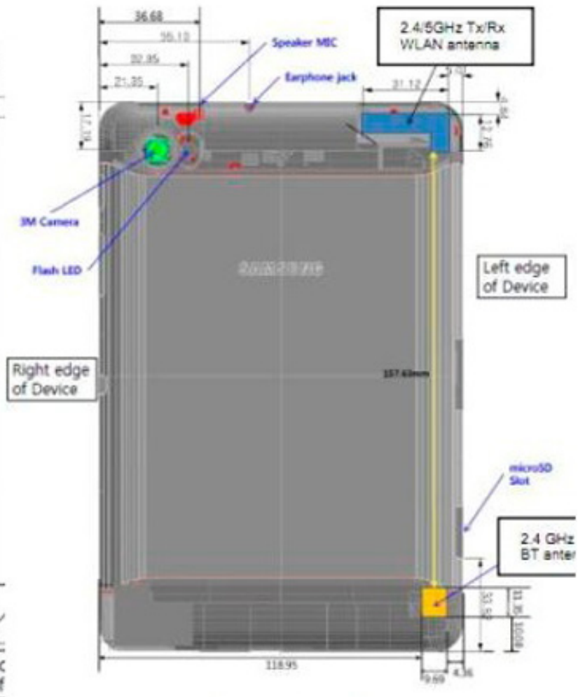
Figure 11-2 Back View of Device
